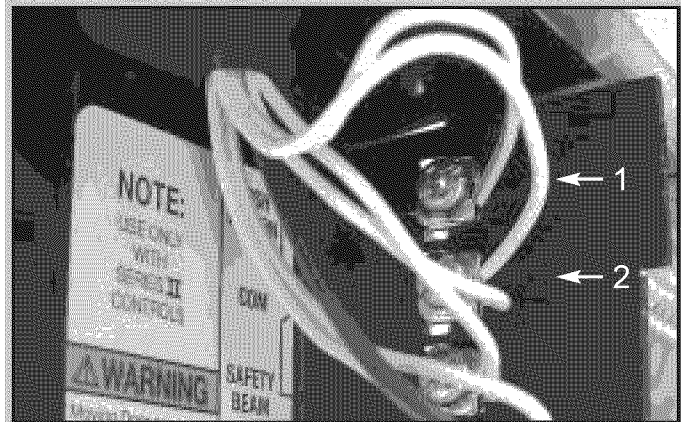
FIG. 5-1 Terminal attachments at power head.
