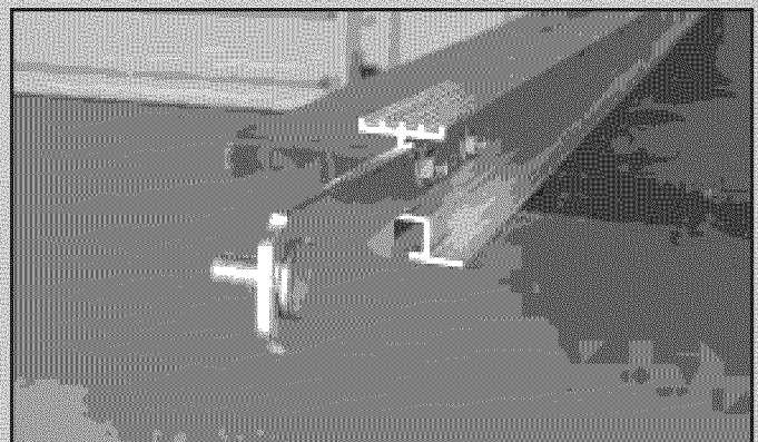
FIG. 1-4 Attach rail strap.
