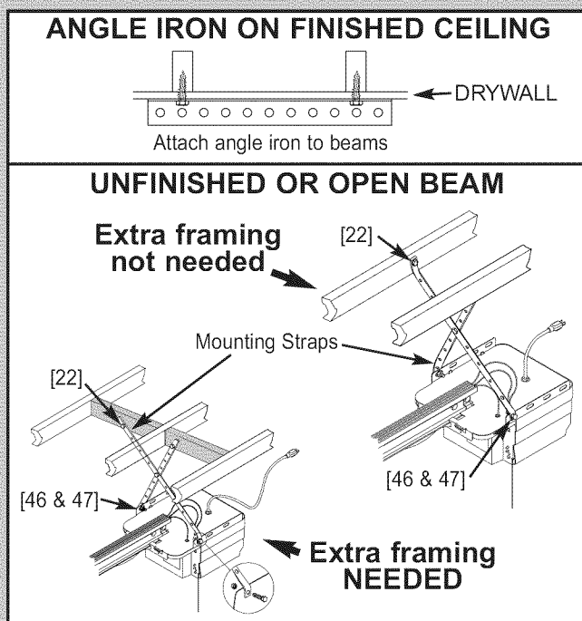
FIG. 2-10 Mounting the power head.
