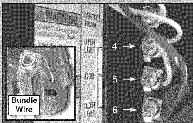
FIG. 1-14 Attach wire at power head terminals.
