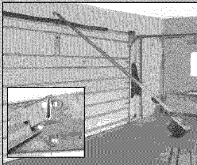
FIG. 2-7 Position assembly.
